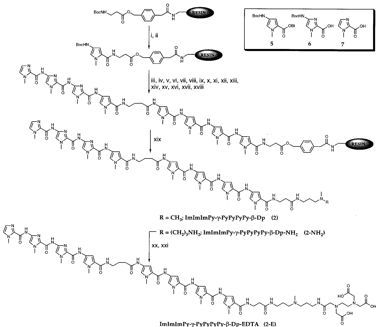
Figure 3. (Box) Pyrrole and imidazole monomers for synthesis of all compounds described here: Boc-pyrrole-OBt ester 5, 7 Boc-imidazole-acid 6, 7 and imidazole-2-carboxylic acid 7. 1a Solid-phase synthetic scheme for ImImImPy-γ-PyPyPyPy-β-Dp, ImImImPy-γ-PyPyPyPy-β-Dp-NH 2 , and ImImImPy-γ-PyPyPyPy-β-Dp-EDTA prepared from commercially available Boc-β-alanine-Pam-resin (0.2 mmol/g): (i) 80% TFA/DCM, 0.4 M PhSH; (ii) BocPy-OBt, DIEA, DMF; (iii) 80% TFA/DCM, 0.4 M PhSH; (iv) BocPy-OBt, DIEA, DMF; (v) 80% TFA/DCM, 0.4 M PhSH; (vi) BocPy-OBt, DIEA, DMF; (vii) 80% TFA/DCM, 0.4 M PhSH; (viii) BocPy-OBt, DIEA, DMF; (ix) 80% TFA/DCM, 0.4 M PhSH; (x) Boc-γ-aminobutyric acid (HBTU, DIEA), DMF; (xi) 80% TFA/DCM, 0.4 M PhSH; (xii) BocPy-OBt, DIEA, DMF; (xiii) 80% TFA/DCM, 0.4 M PhSH; (xiv) BocIm-OBt (DCC/HOBt), DIEA, DMF; (xv) 80% TFA/DCM, 0.4 M PhSH; (xvi) BocIm-OBt (DCC/HOBt), DIEA, DMF; (xvii) 80% TFA/DCM, 0.4 M PhSH; (xviii) imidazole-2-carboxylic acid (HBTU/DIEA); (xix) (( N,N -dimethylamino)propyl)amine or 3,3'-diamino- N -methylpropylamine, 55 °C; (xx) EDTA-dianhydride, DMSO/NMP, DIEA, 55 °C; (xxi) 0.1 M NaOH.
