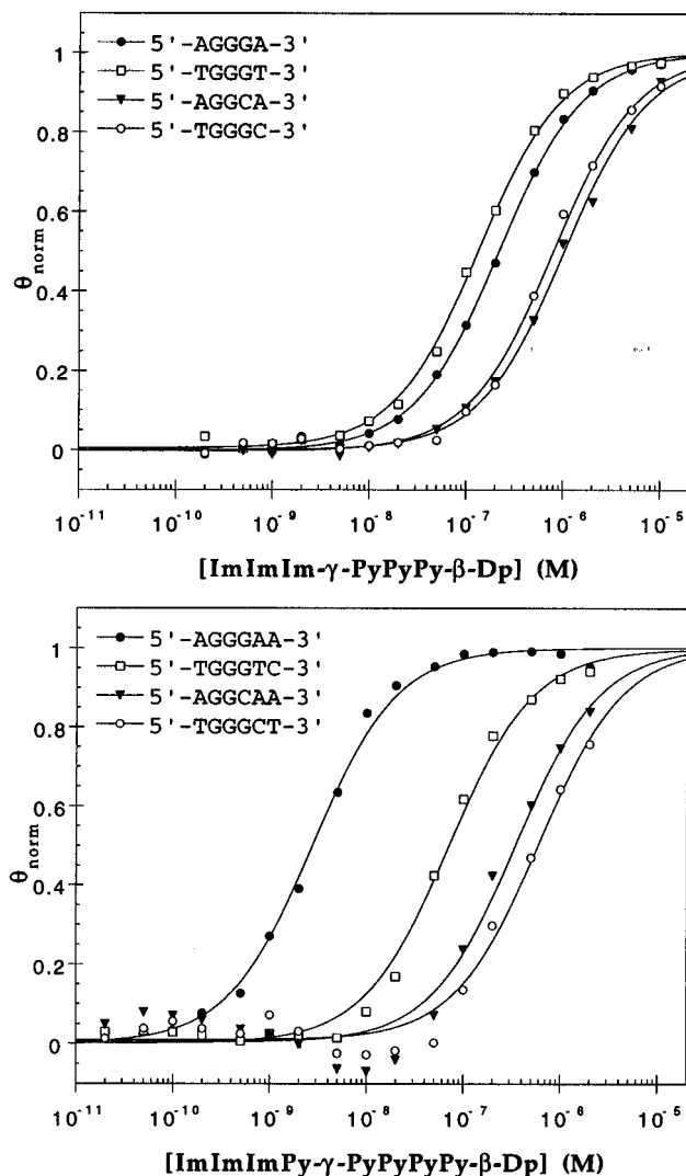
Figure 7. Data from the quantitative DNase I footprint titration experiments for the two polyamides, ImImIm- \gamma -PyPyPy- \beta -Dp (top) and ImImImPy- \gamma -PyPyPy- \beta -Dp (bottom), in complex with the designated sites. The \theta_{\text{norm}} points were obtained using photostimulable storage phosphor autoradiography and processed as described in the Experimental Section. The data points for 5'-AGGGA(A)-3', 5'-TGGGT(C)-3', 5'-AGGCA(A)-3', and 5'-TGGGC(T)-3' sites are indicated by filled circles ( \bullet ), open squares ( \square ), filled inverted triangles ( \blacktriangledown ), and open circles ( \circ ), respectively. The solid curves are the best-fit Langmuir binding titration isotherms obtained from the nonlinear least-squares algorithm using eq 2.
